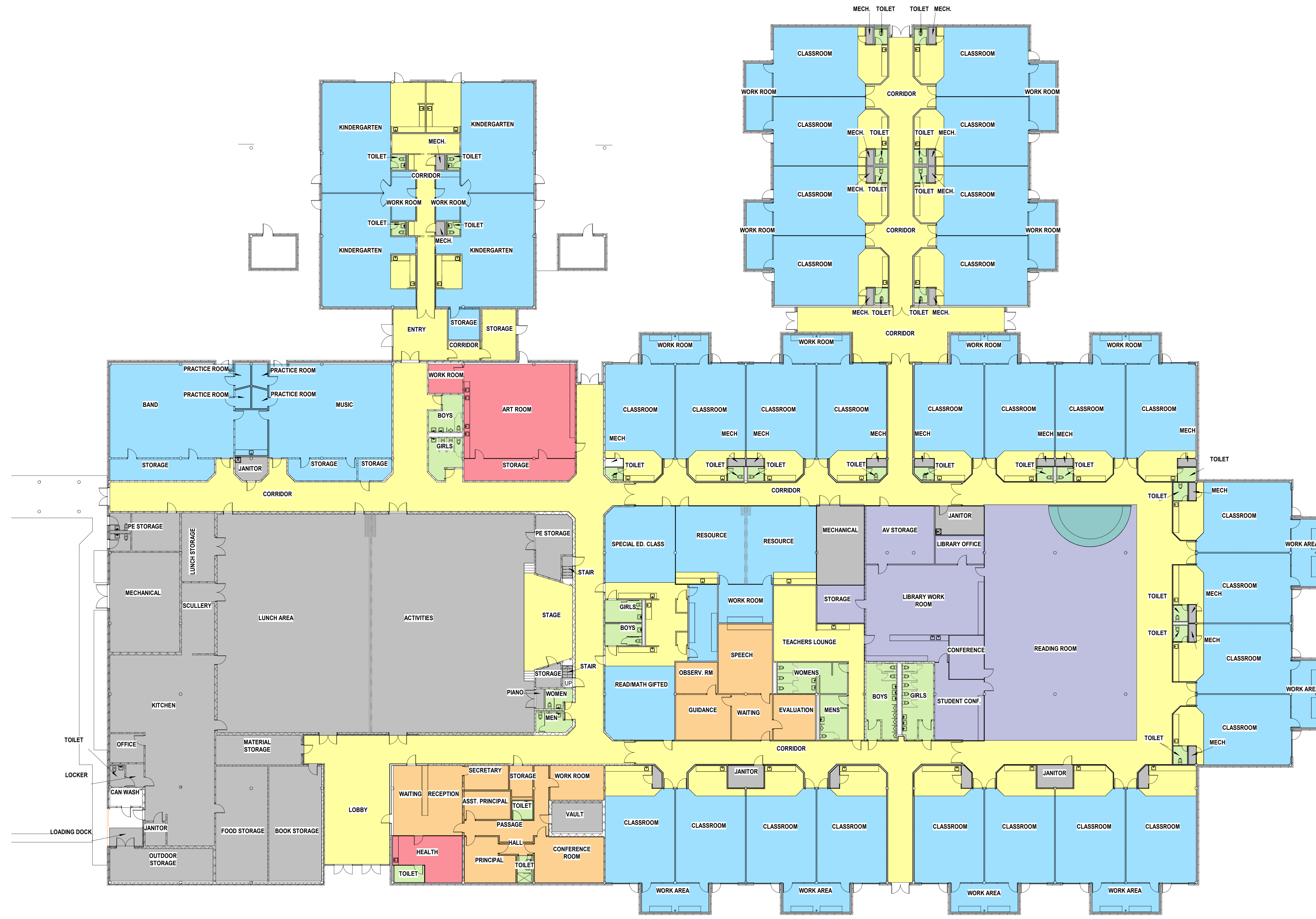
1 EXISTING BUILDING - FLOOR FINISH PLAN COLOR CODED 1/16" = 1'-0"
